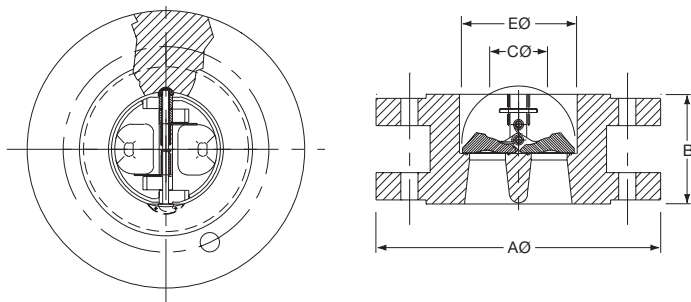
FLANGE DETAIL
